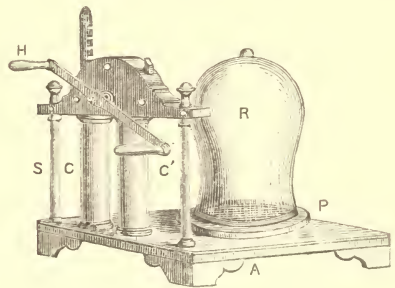
FIG. 2.—Double-barrel Air Pump.
